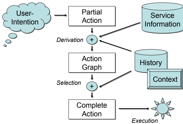
Figure 1. A user intention is transformed into a complete action by selecting the optimal action (action graph) matching the user intention, using the knowledge about available services, the context information and the execution history.
